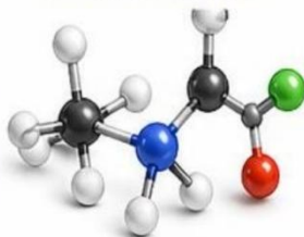
Choline chloride
